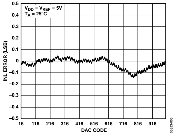
Figure 6. Typical AD5611 INL
