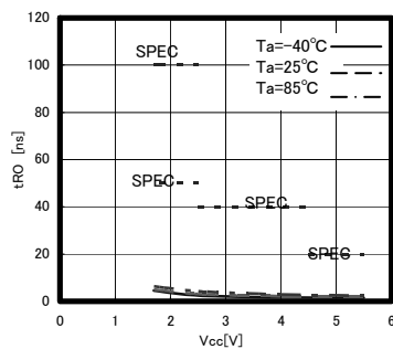
Fig.30 Output rise time t_{RO}
