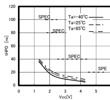
Fig.29 Time from HOLDB to output change t_{HPD}
