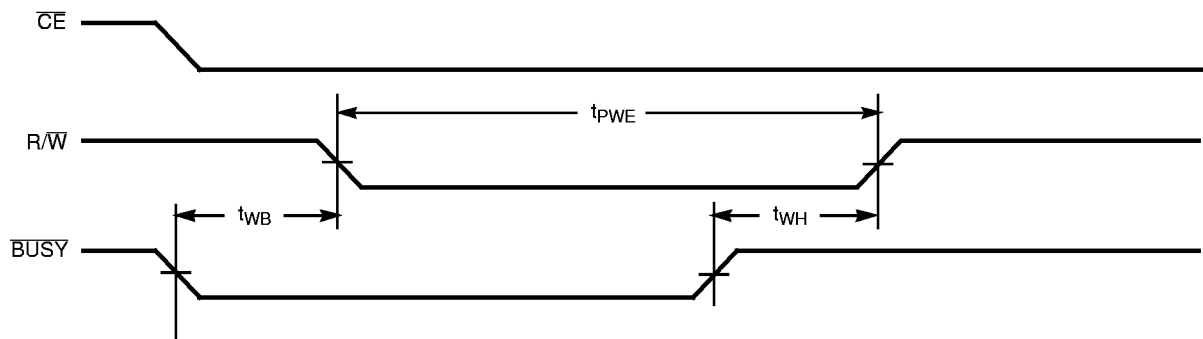
Busy Timing Diagram No.3 (Write with \overline{\text{BUSY}} , Slave:CY7B146)
