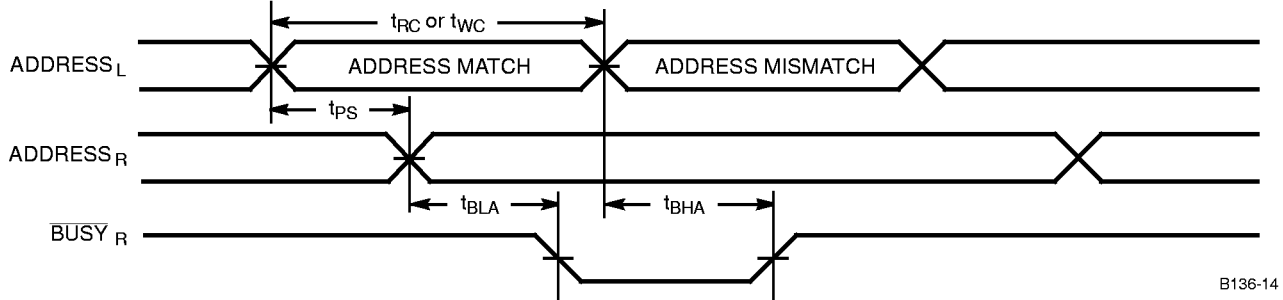
Busy Timing Diagram No.2 (Address Arbitration)
