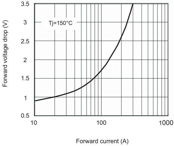
Fig.1 Forward characteristic
