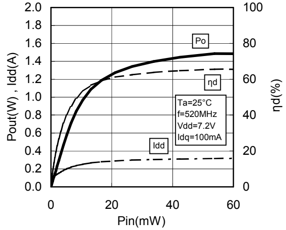
Pin-Po CHARACTERISTICS
