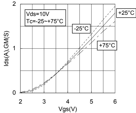
Vgs-Ids CHARACTERISTICS 2
