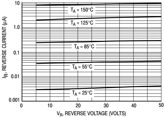
Figure 5. Leakage Current
