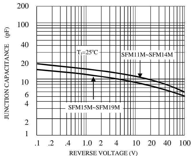
FIG. 6-TYPICAL JUNCTION CAPACITANCE
