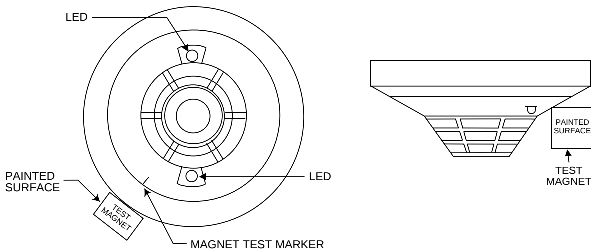
Figure 2. Views showing position of test magnet.
