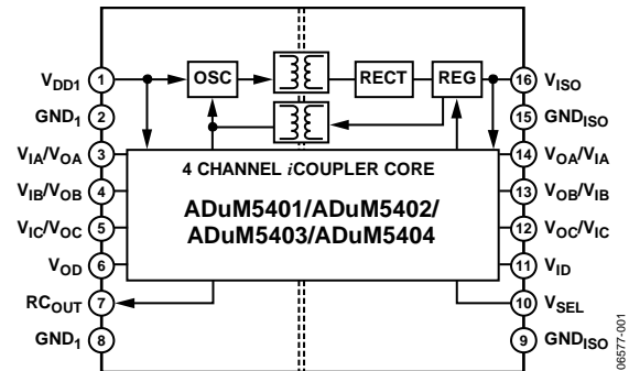
Figure 1. ADuM5401/ADuM5402/ADuM5403/ADuM5404
