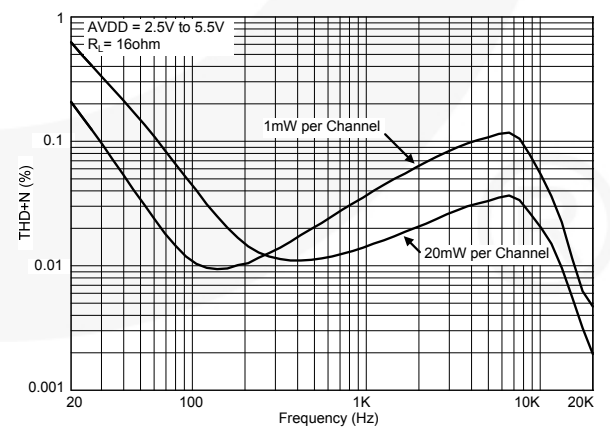
Figure 15. THD vs. Frequency at 16Ω
