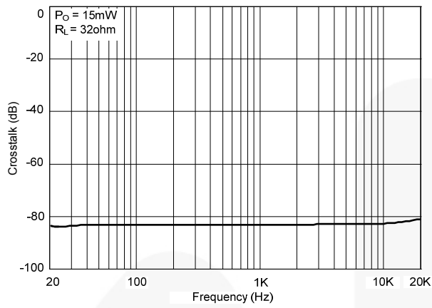
Figure 16. Crosstalk vs. Frequency at 32Ω
