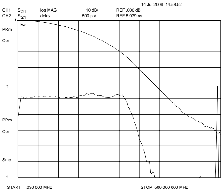
Passband Amplitude & Group Delay (10 dB/div and 0.5 nsec/div)
