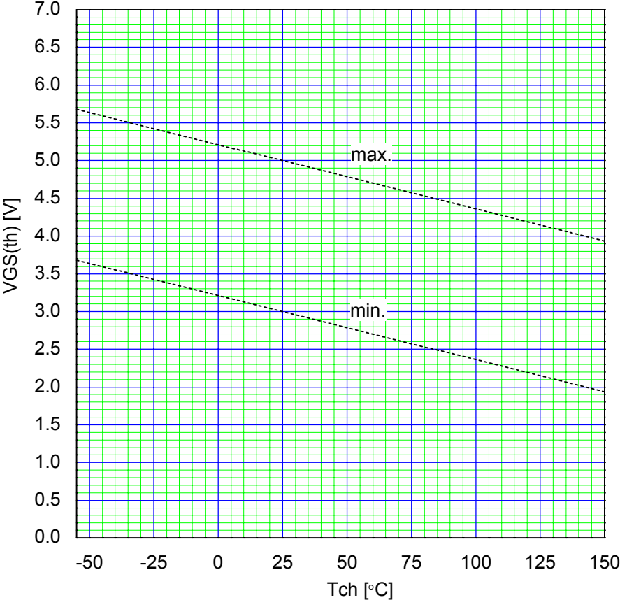
Gate Threshold Voltage vs. T ch V GS(th) =f(T ch ):V DS =V GS ,I D =250A
