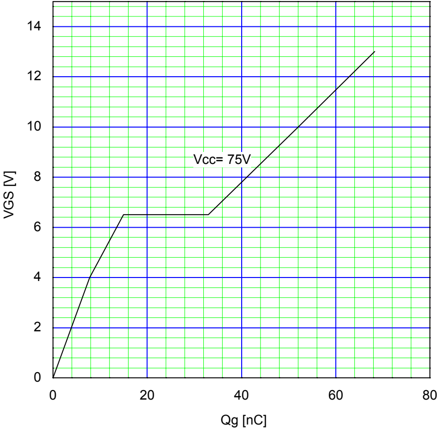
Typical Gate Charge Characteristics V GS =f(Q g ):I D =40A,T ch =25°C
