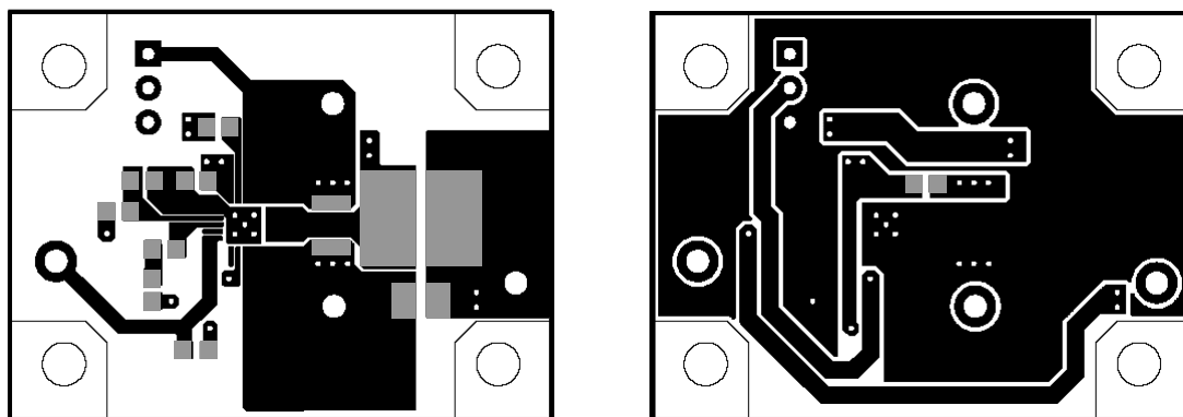
Fig.36 Layout diagram
