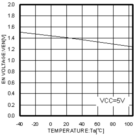
Fig.11 T_a - V_{EN}
