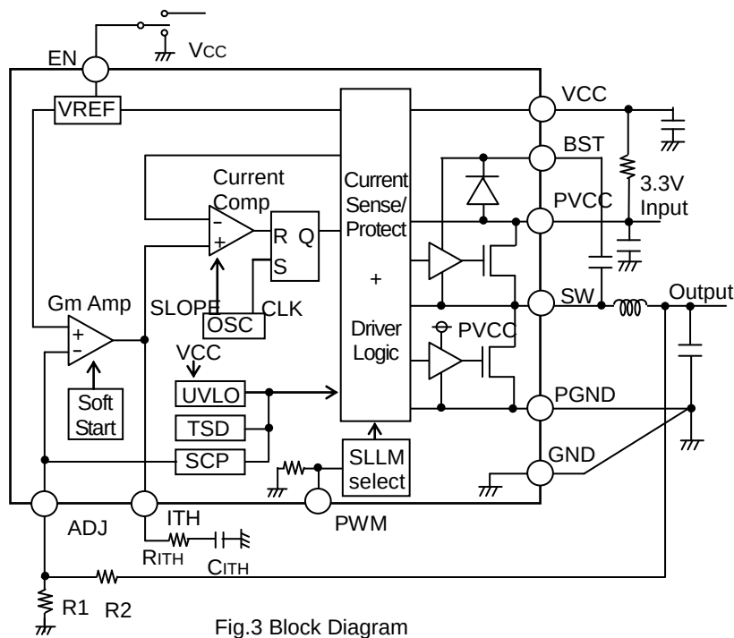
Fig.3 Block Diagram
