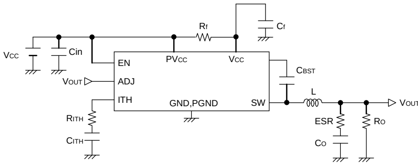
Fig.33 Typical application
