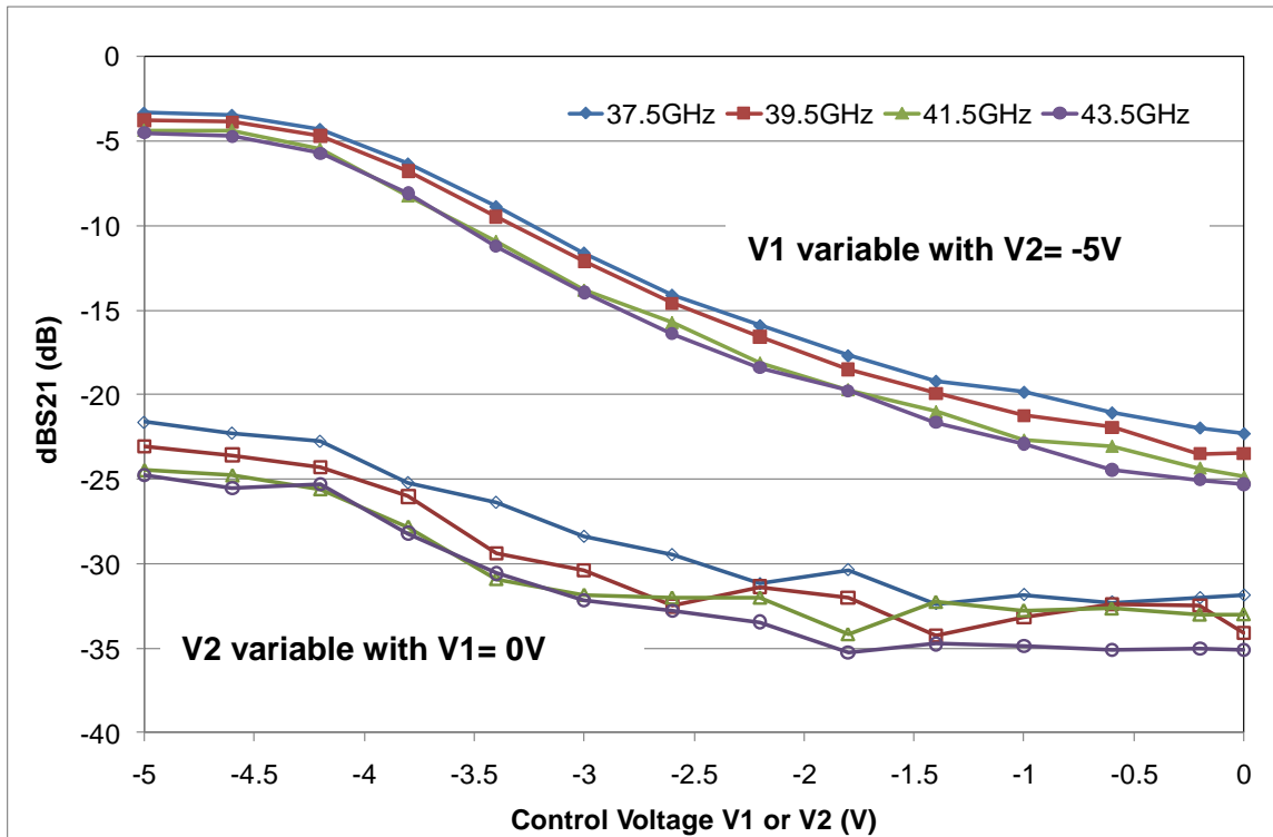
Gain versus control voltage
