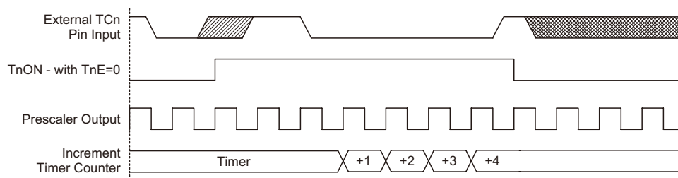
Pulse Width Capture Mode Timing Chart (TnE=0)
