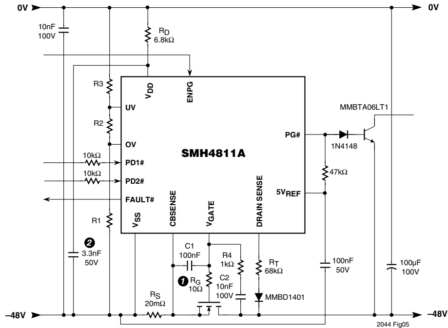
Figure 5. Changing Polarity of Power Good Output
