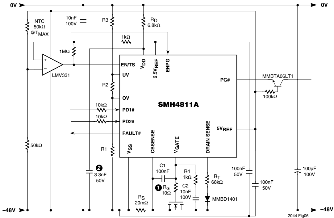
Figure 6. Overtemperature Shutdown
