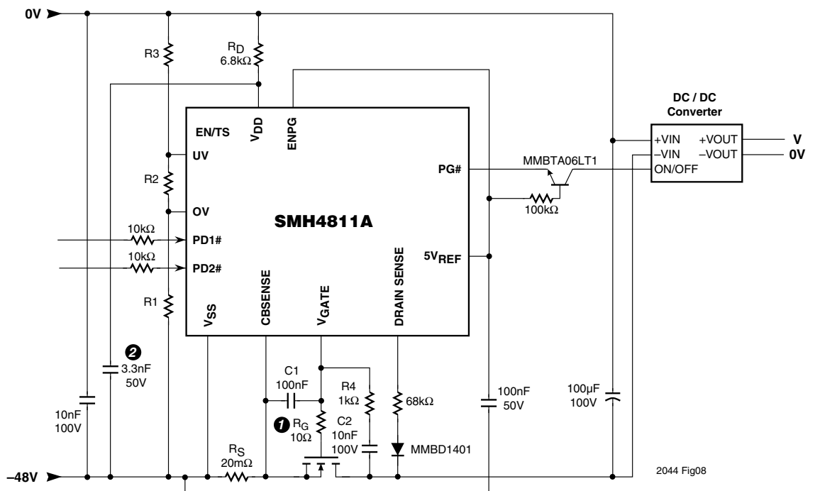
Figure 8. Typical Application with DC/DC Converter
