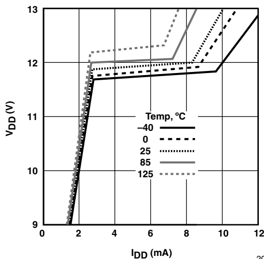
Figure 4. Shunt Regulator Voltage vs. I_{DD} at Various Temperatures
