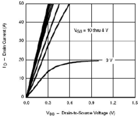
Output Characteristics
