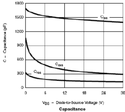
Capacitance
