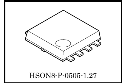
Weight: 0.068 g (typ.)
