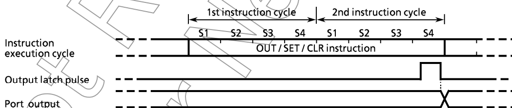
Figure 3-2. Output Timing
