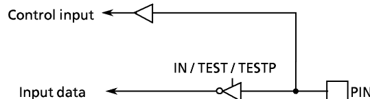
Figure 3-6. Port KE
