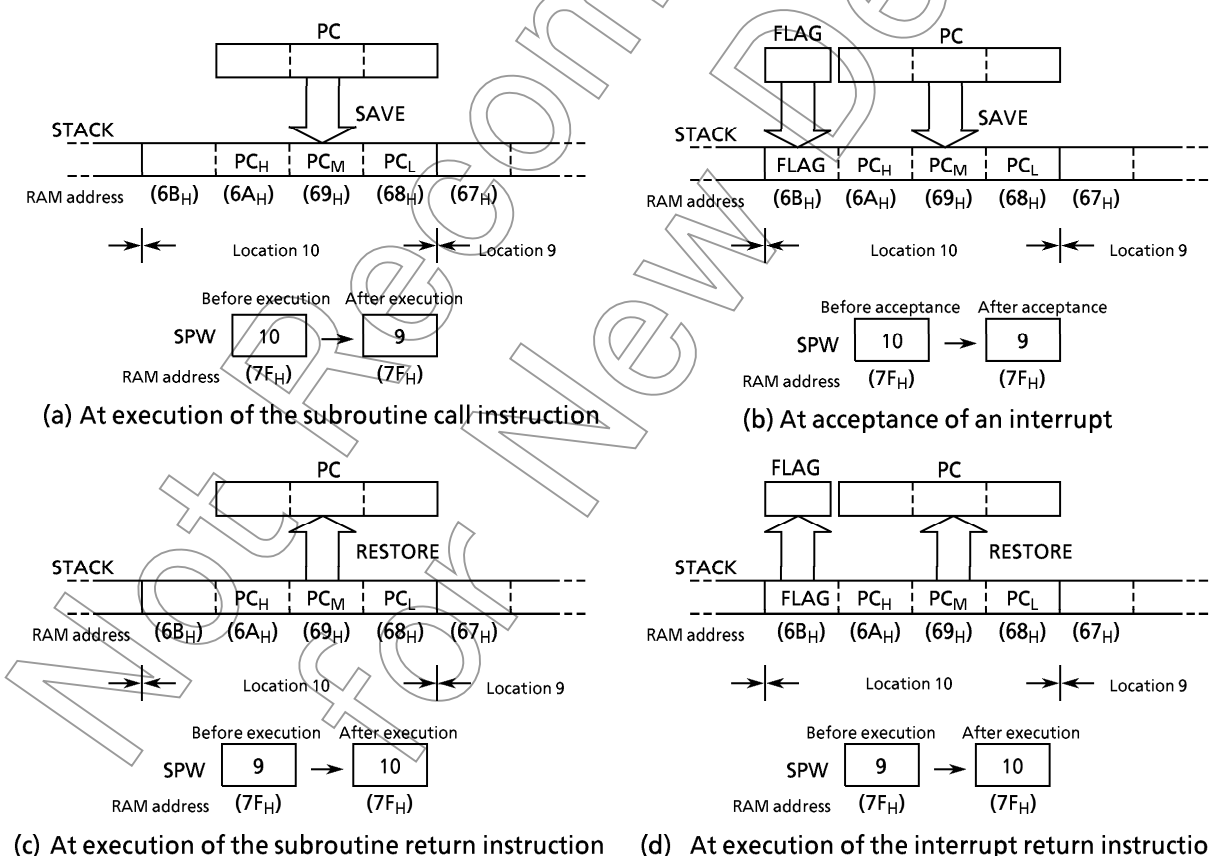
Figure 2-8. Accessing Stack (Save / Restore at the TMP47C202)
