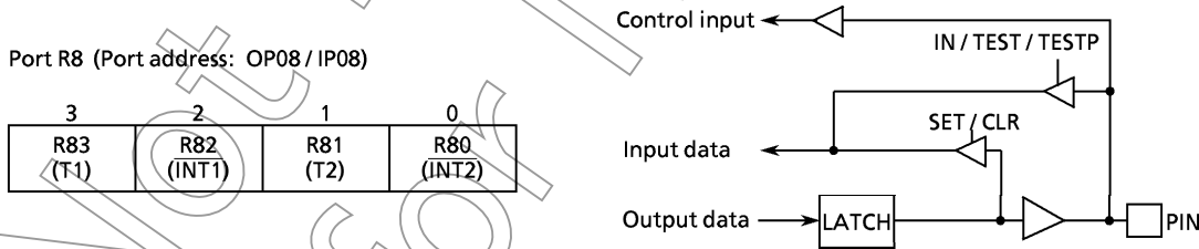
Figure 3-7. Port R8
