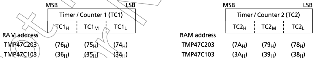
Figure 3-11. The Count registers of the Timer / Counters (TC1, TC2)
