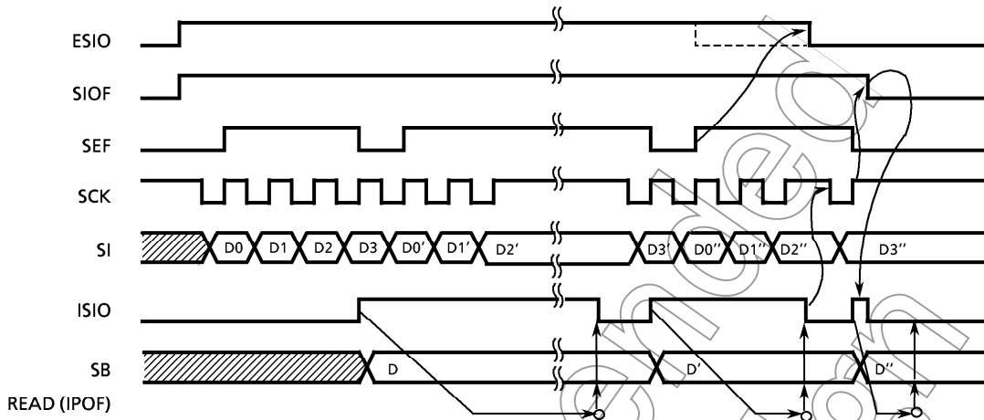
(a) Internal-clock-based operation, trailing-edge-shift (with wait)
