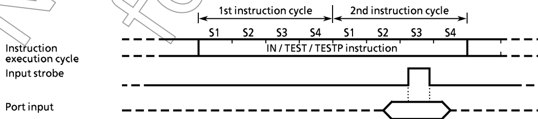
Figure 3-1. Input Timing
