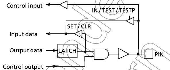
Figure 3-8. Port R9
