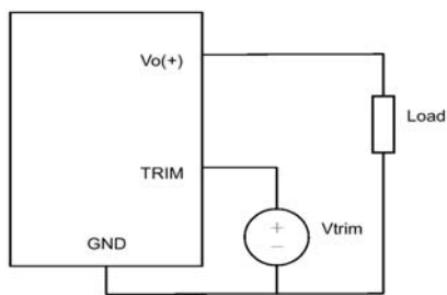
Figure 30: Circuit configuration for programming output voltage using external voltage source
