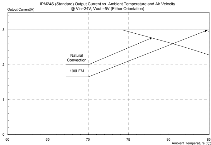
Figure 34: Output current vs. ambient temperature and air velocity @Vin=24V, Vout=5V(Either Orientation)
