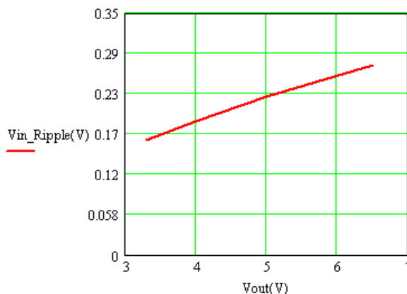
Figure 26: Input ripple voltage for various output models, I_o = 3A ( C_{in} = 2x100\mu F electrolytic capacitors 1x3.3µF ceramic capacitors at the input)
