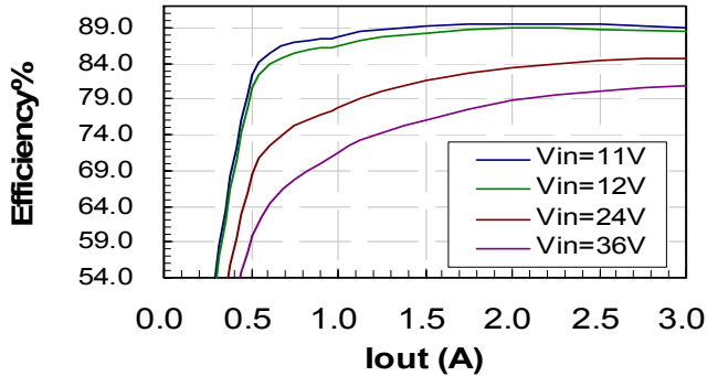
Figure 1: Converter efficiency vs. output current (3.30V output voltage)
