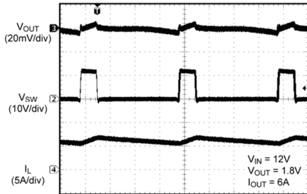
Switching Waveforms; I_{OUT} = 6A
