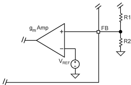
Figure 7. Voltage-Divider Configuration
