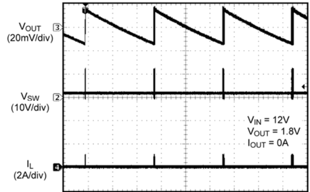
Switching Waveforms; I_{OUT} = 0A
