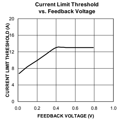
Figure 5. MIC26603 Current Limit Foldback Characteristic
