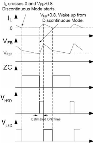
Figure 4. MIC26603 Control Loop Timing (Discontinuous Mode)
