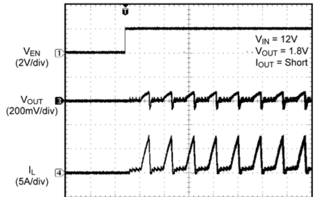
Enable into Short Circuit
