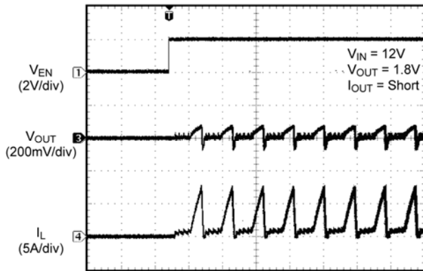
Enable into Short Circuit
