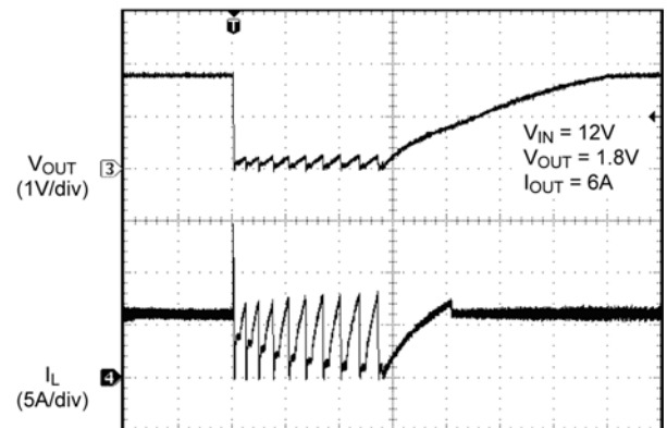
Output Recovery from Short Circuit
