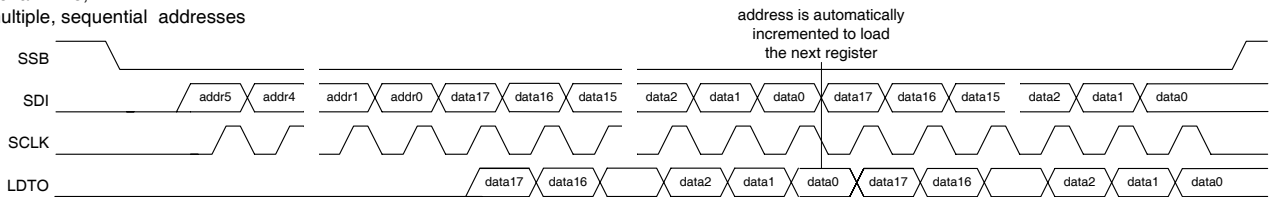
Serial Write, multiple, sequential addresses
