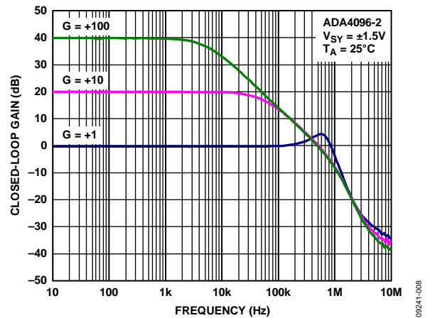
Figure 8. Closed-Loop Gain vs. Frequency
