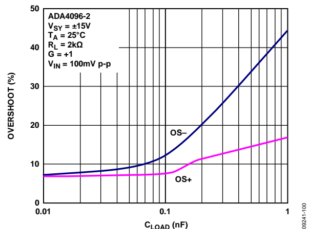
Figure 44. Overshoot vs. Load Capacitance
