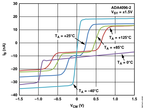
Figure 5. Input Bias Current vs. V CM and Temperature
