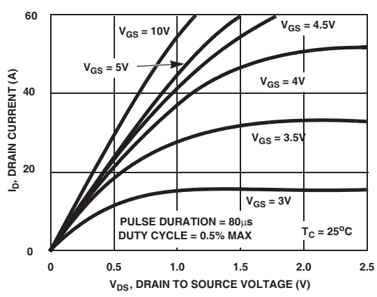
Figure 8. Saturation Characteristics
