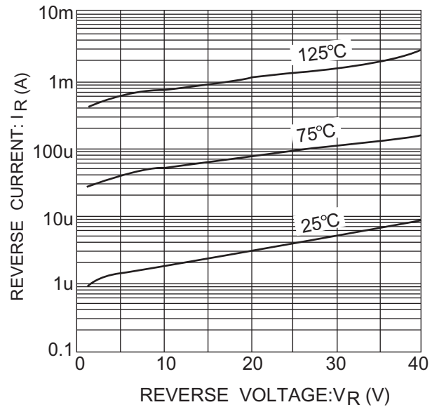
Fig.2 Reverse characteristics
