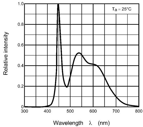
Fig. 8.4 Wavelength characteristic
