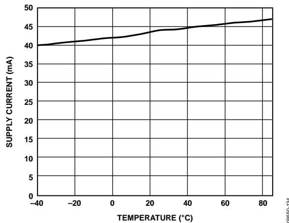
Figure 34. Supply Current (VGA2 Switch Enabled) over Temperature
