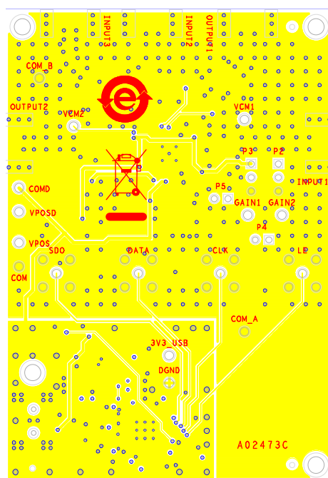
Figure 73. Silkscreen Bottom
