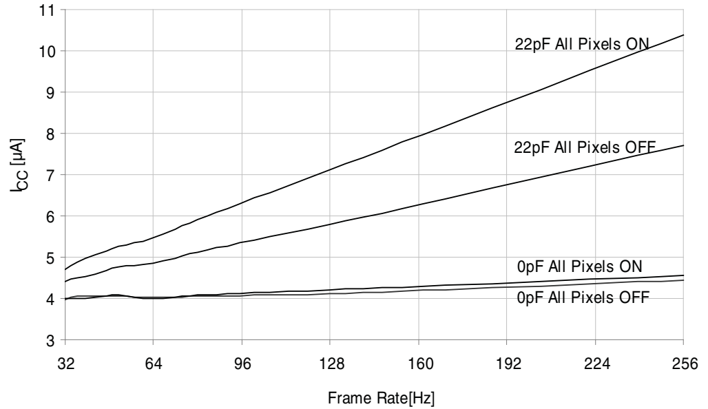
Figure 37-74. I_{CC} vs. Frame Rate
