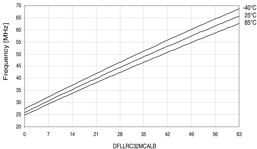
Figure 37-67. 32MHz internal oscillator frequency vs. CALB calibration value. V_{CC} = 3.0V , DFLL enabled.
