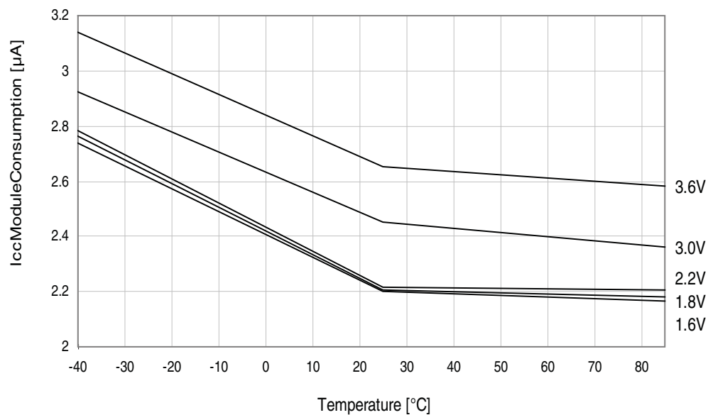
Figure 37-78. Psave LCD LP 32Hz vs. Temperature
