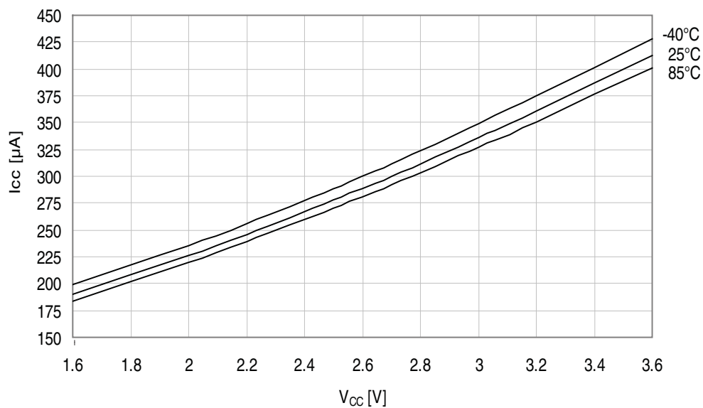
Figure 37-8. Idle mode supply current vs. V_{CC} . f_{SYS} = 2MHz internal oscillator.
