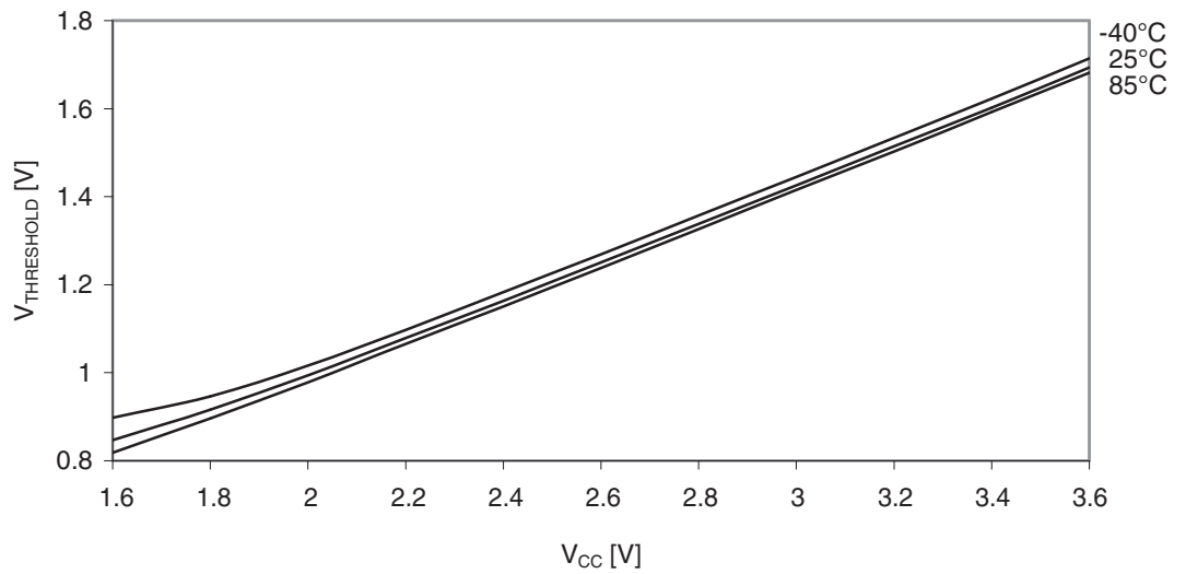
Figure 37-22. I/O pin input threshold voltage vs. V_{CC} .
