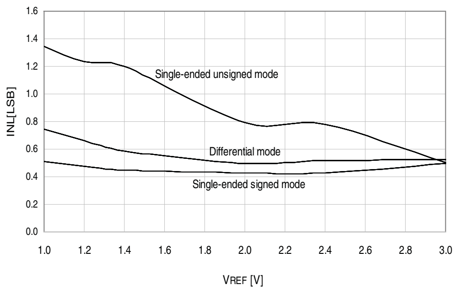
Figure 37-24. INL error vs. external V_{REF} .
