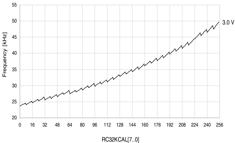
Figure 37-57. 32.768kHz internal oscillator frequency vs. calibration value. V CC = 3.0V, T = 25°C.
