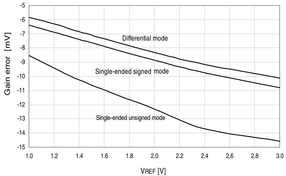
Figure 37-30. Gain error vs. V_{REF} . T = 25°C, V_{CC} = 3.6V , ADC sample rate = 300kpsps.
