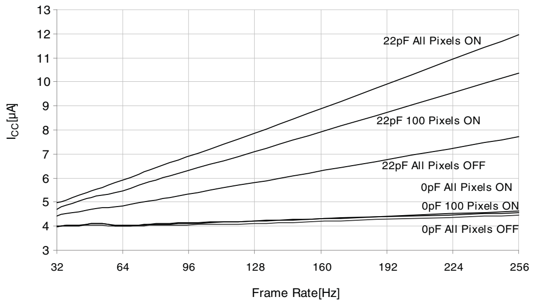
Figure 37-74. I_{CC} vs. Frame Rate
