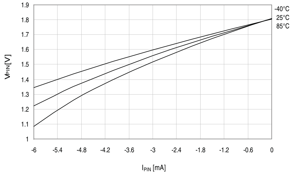
Figure 37-16. I/O pin output voltage vs. source current.
