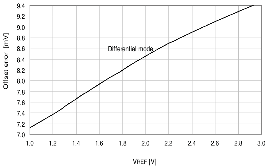
Figure 37-32. Offset error vs. V_{REF} .
