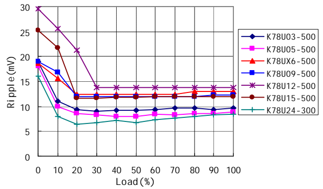
Ripple VS Load curve (Vin=Vmax)
