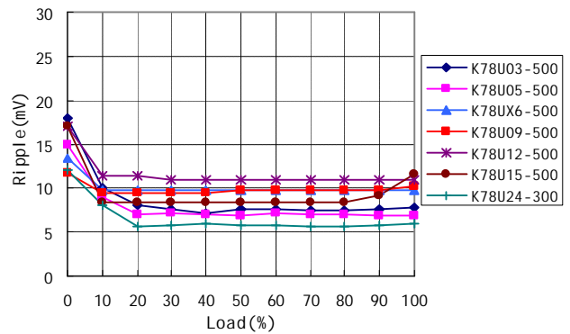
Ripple VS Load curve (Vin=Vmin)
