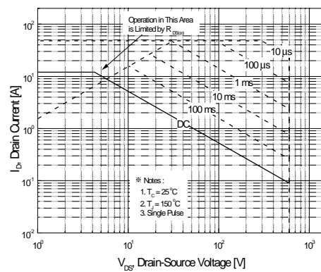
Fig. 10. Maximum safe operating area (TO-220F)
