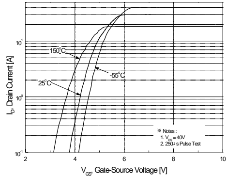
Fig. 2. Transfer characteristics
