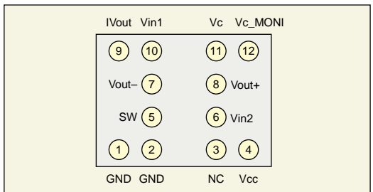
■ Figure 3 CXA2701GA Pin Configuration
