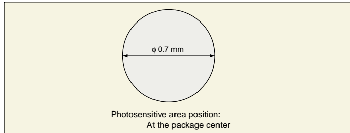
■ Figure 5 CXA2701GA Acceptance Pattern Dimensions
