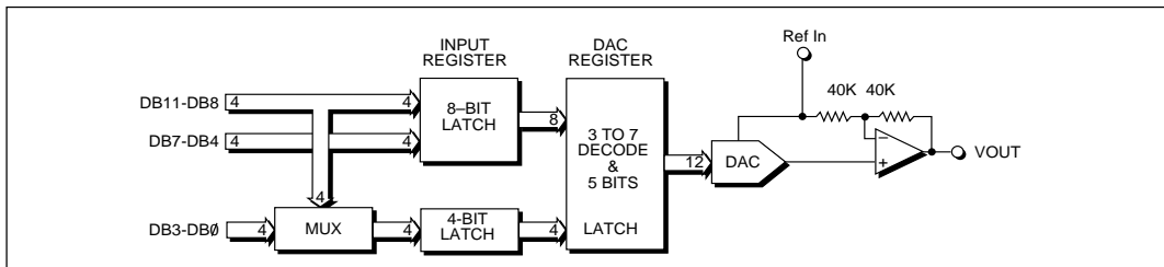
Figure 1. Detailed Block Diagram (only one DAC shown)
