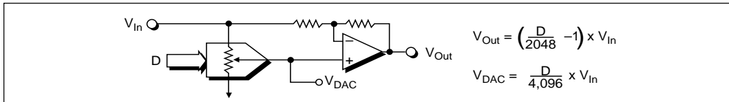
Figure 2. Transfer Function
