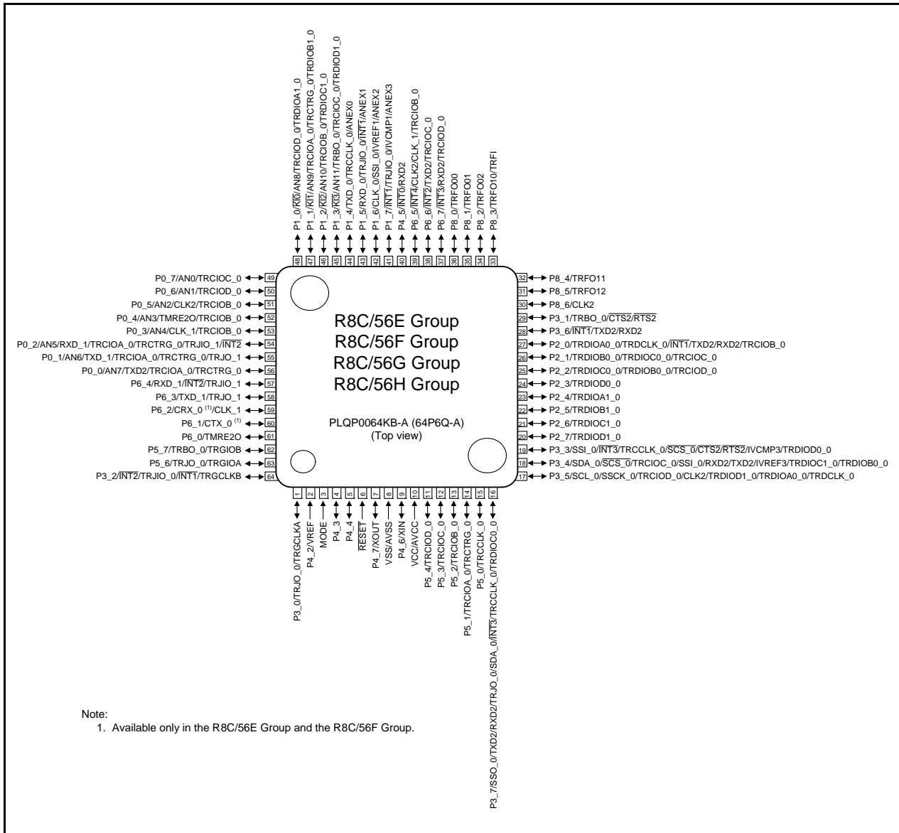
Figure 1.6 Pin Assignment (Top View)
