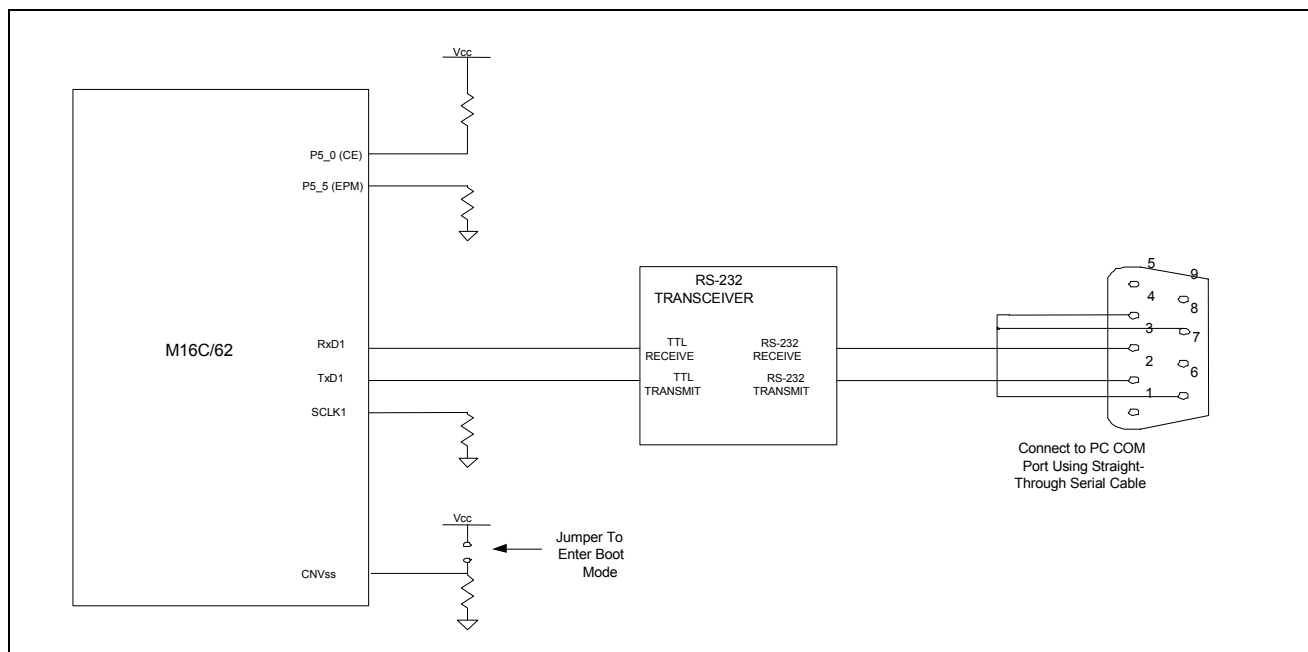
Figure 1 Typical Connection for Asynchronous Serial Programming
