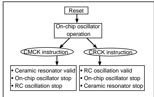
Fig. 59 Switch to ceramic oscillation/RC oscillation
