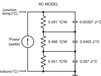
FIGURE 25b. TRANSIENT THERMAL IMPEDANCE MODEL
