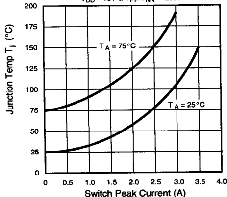
Junction Temp T_j vs Switch Peak Current V_{SIG} Freq = 10KHz & Duty Cycle = 0.1% V_{DD} = 15V & V_{PP}/V_{NN} = \pm 80V
