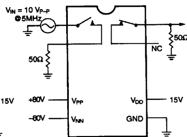
Crosstalk
