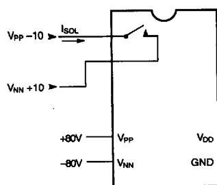
Switch OFF Leakage
