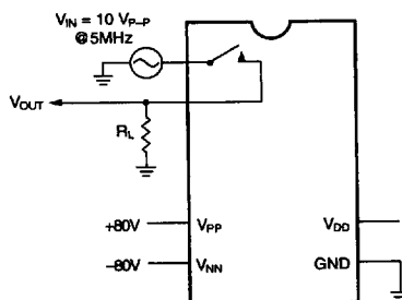
OFF Isolation
