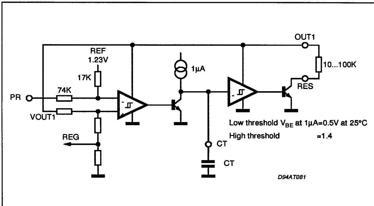
Figure 3: Reset Generator
