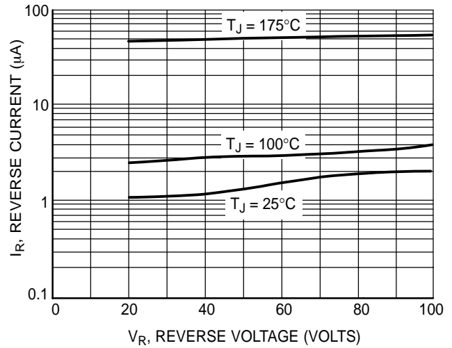
Figure 2. Maximum Reverse Current
