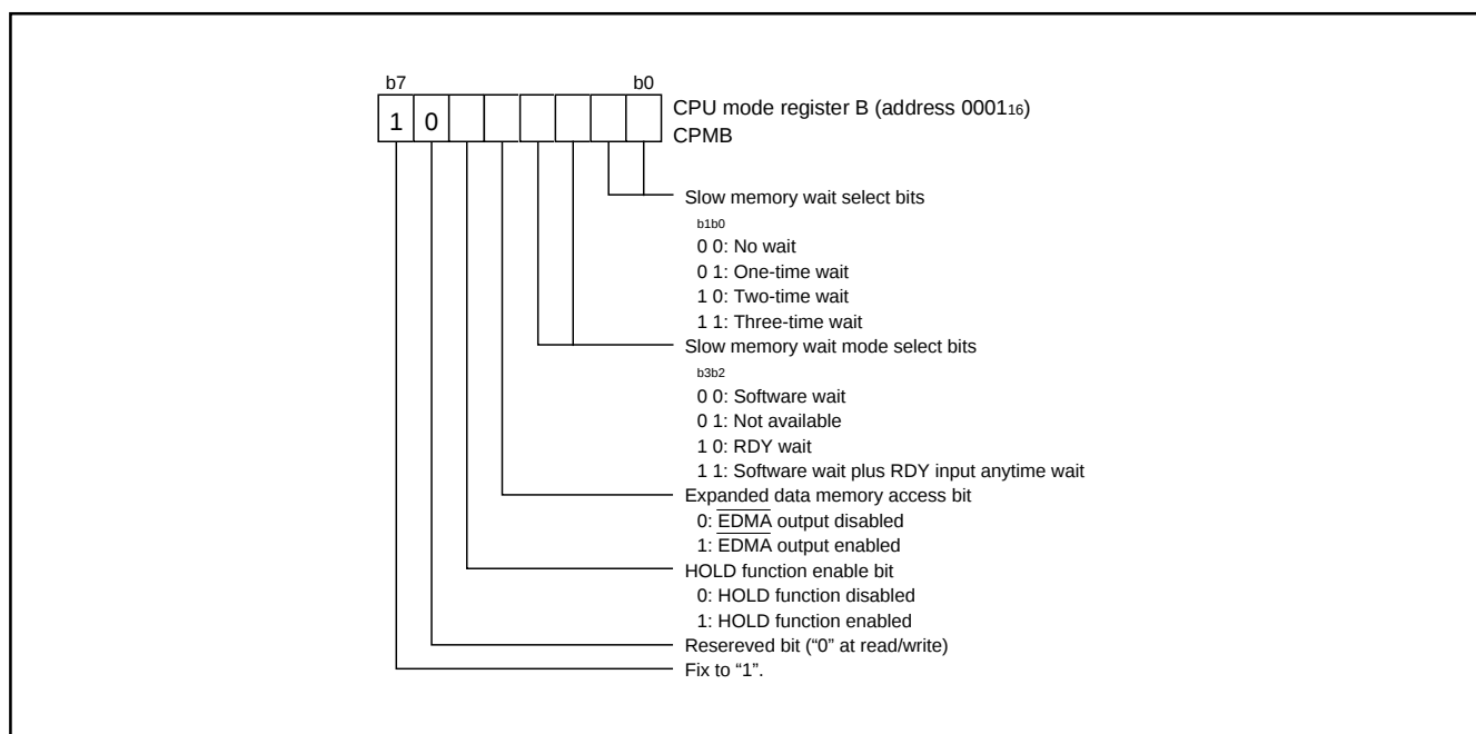
Fig. 71 Structure of CPU mode register B
