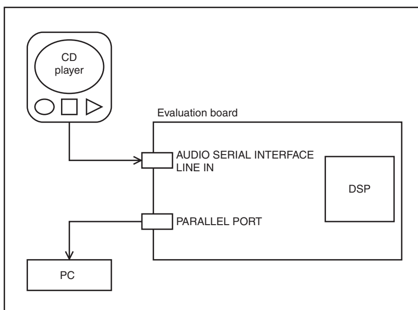
Figure 1-2. System Configuration Example
