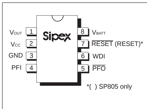
Figure 10. Pinout
