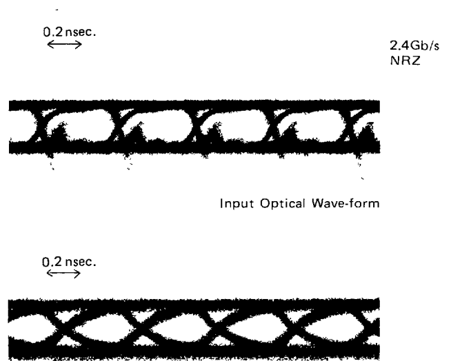
Fig. 2 Pulse Response
