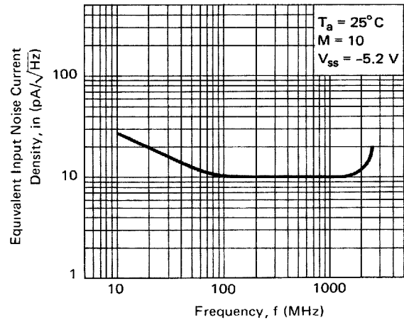
Fig. 4 Equivalent Input Noise Current Density
