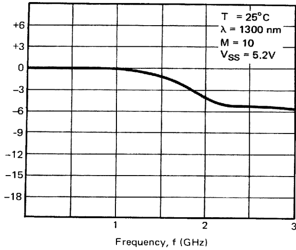
Fig. 1 Frequency Response
