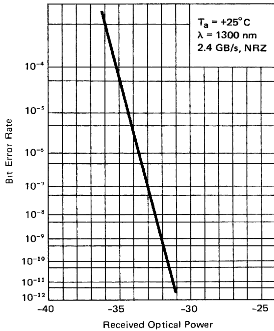
Fig. 3 Bit Error Rate Characteristics
