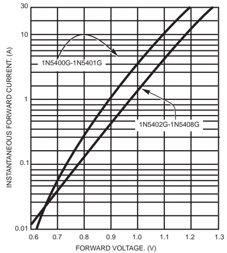
FIG.5- TYPICAL FORWARD VOLTAGE
