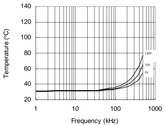
Figure 32. IRS2106S vs. Frequency (IRFBC20), R_{gate}=33 \Omega, V_{CC}=15 V
