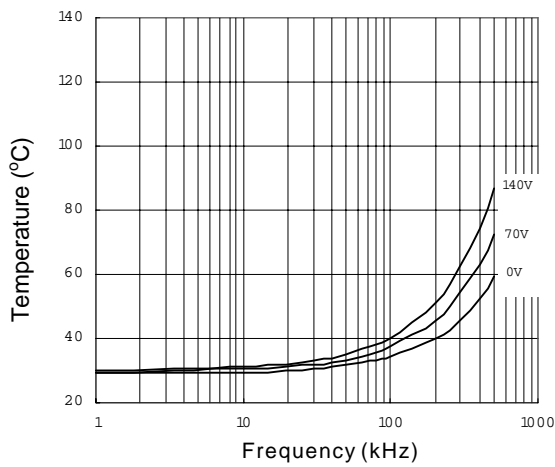
Figure 25. IRS2106 vs. Frequency (IRFBC30), R_{gate}=22 \Omega , V_{CC}=15 V
