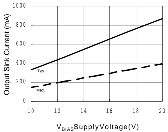
Figure 22B. Output Sink Current vs. Supply Voltage
