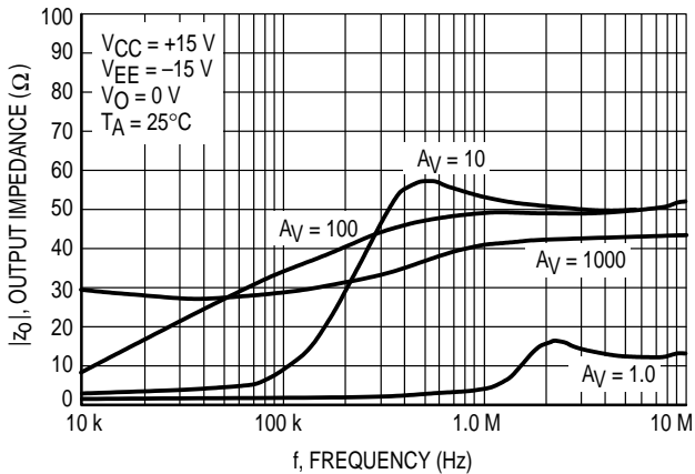
Figure 24. Output Impedance versus Frequency
