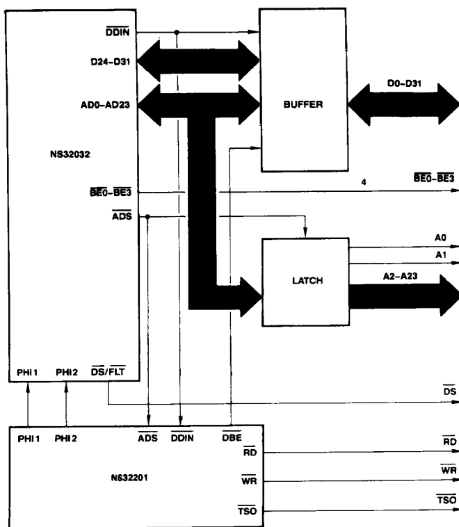
FIGURE 3-6. Bus Connections
