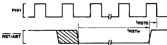
FIGURE 4-26. Non-Power-On Reset
