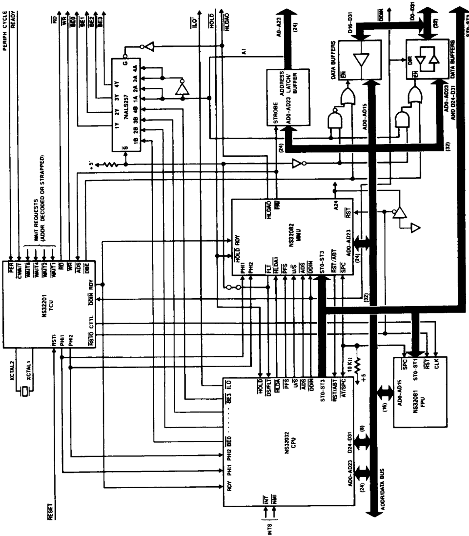
FIGURE B-1. System Connection Diagram
