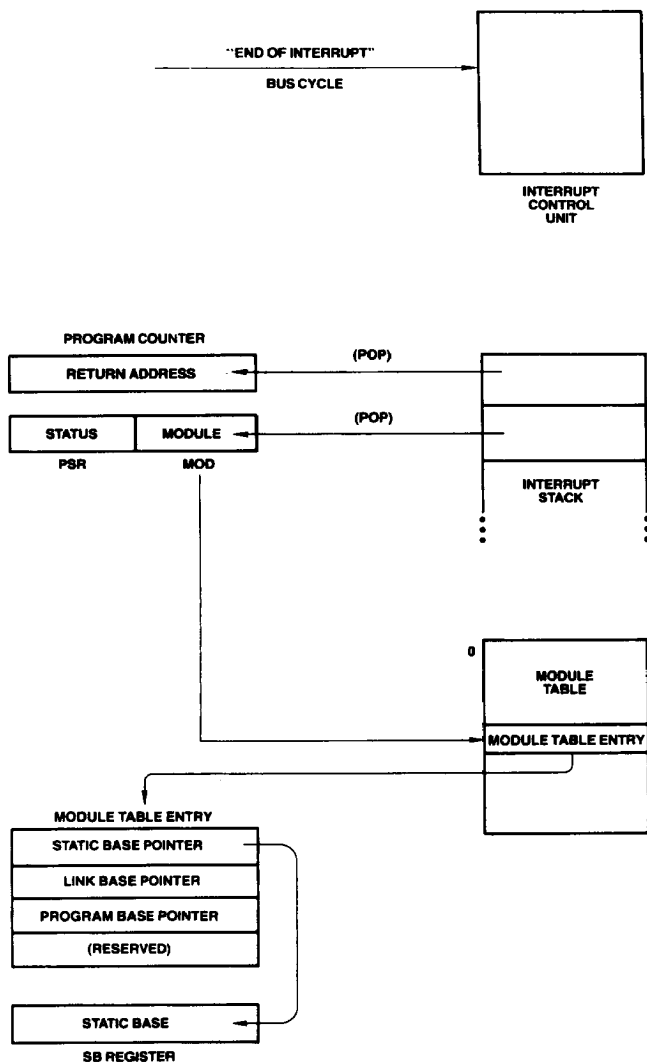
FIGURE 3-25. Return from Interrupt (RETI) Instruction Flow
