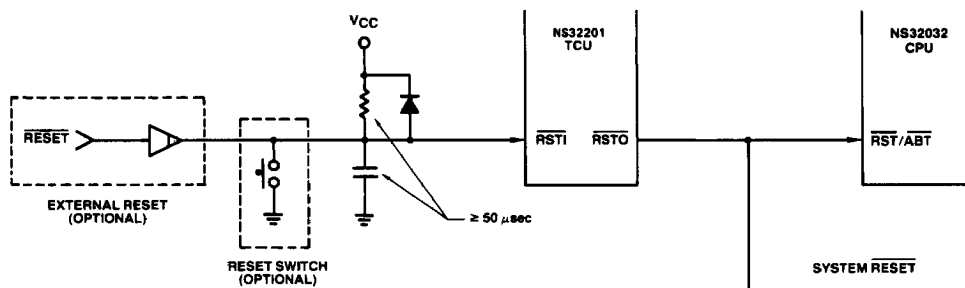
FIGURE 3-5a. Recommended Reset Connections, Non-Memory-Managed System
