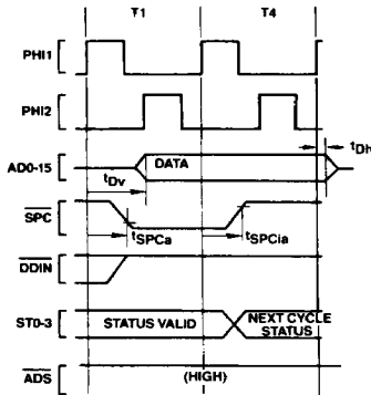
FIGURE 4-13. Slave Processor Write Timing
