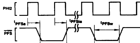
FIGURE 4-18. Relationship of PFS to Clock Cycles
