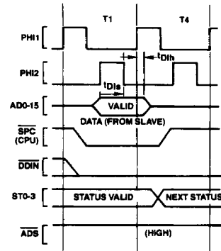
FIGURE 4-14. Slave Processor Read Timing
