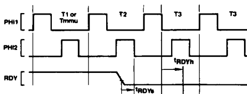
FIGURE 4-11. Ready Sampling (CPU Initially READY)
