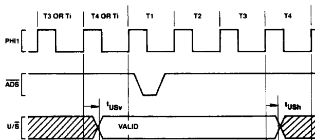
FIGURE 4-22. \overline{\text{U/S}} Relationship to Any Bus Cycle — Guaranteed Valid Interval
