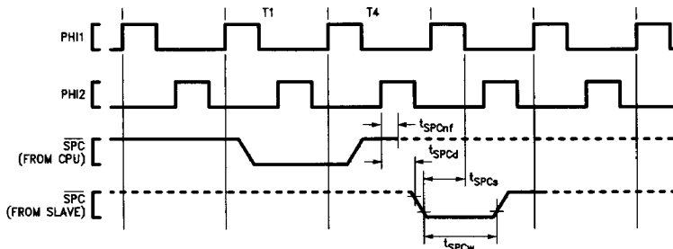
FIGURE 4-15. \overline{SPC} Timing
