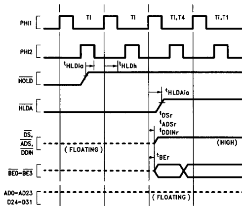
FIGURE 4-8. Release from \overline{\text{HOLD}}
