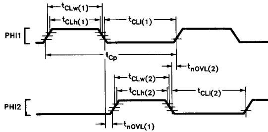
FIGURE 4-17. Clock Waveforms
