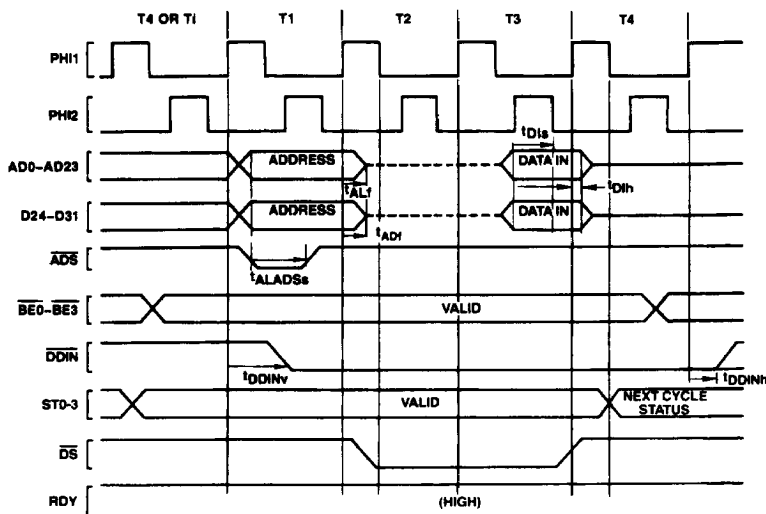
FIGURE 4-5. Read Cycle
