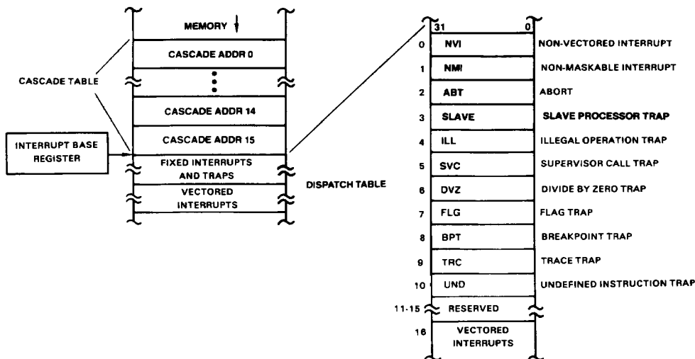
FIGURE 3-22. Interrupt Dispatch and Cascade Tables
