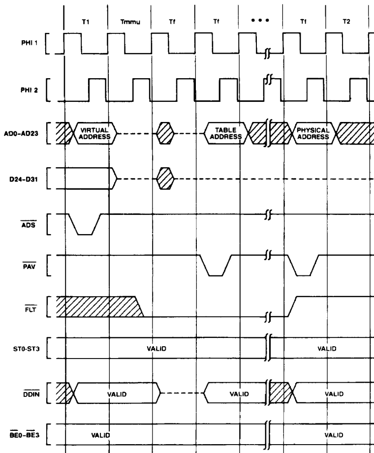
FIGURE 3-19. \overline{\text{FLT}} Timing
