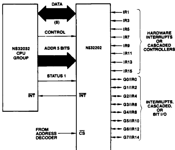
FIGURE 3-26. Interrupt Control Unit Connections (16 Levels)
