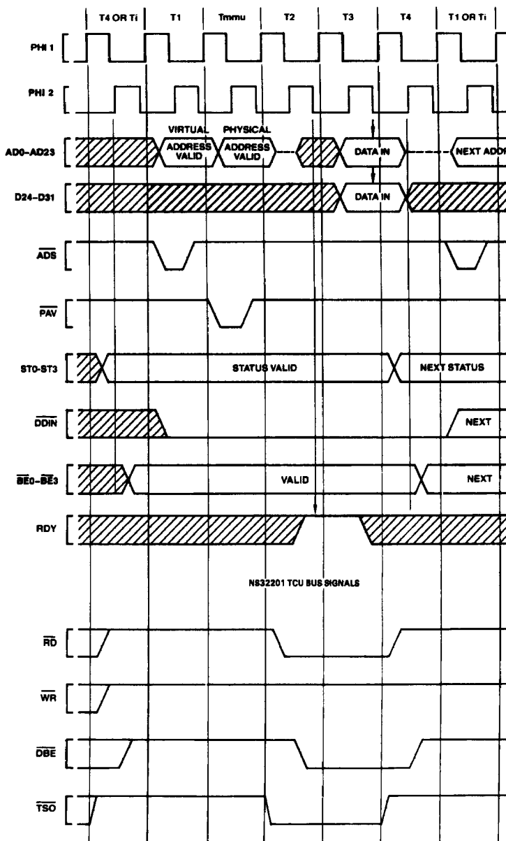
FIGURE 3-17. Memory-Managed Read Cycle
