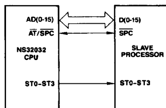
FIGURE 3-12. Slave Processor Connections
