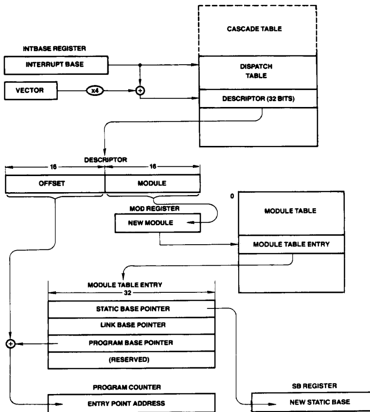
FIGURE 3-23. Interrupt/Trap Service Routine Calling Sequence
