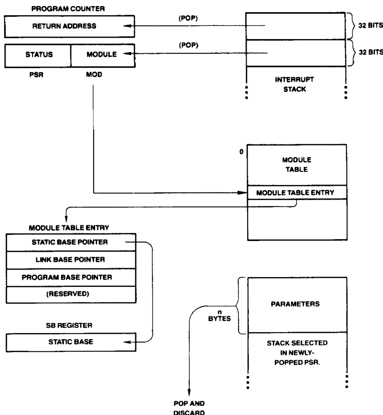
FIGURE 3-24. Return from Trap (RETT n) Instruction Flow
