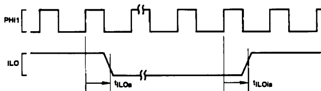
FIGURE 4-21. Relationship of \overline{\text{ILO}} to Any Clock Cycle
