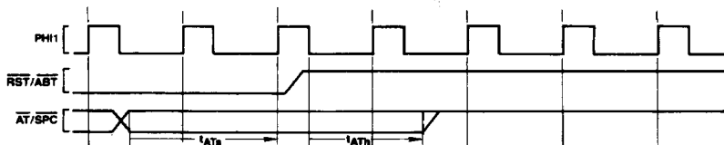
FIGURE 4-16. Reset Configuration Timing
