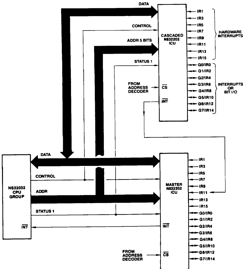
FIGURE 3-27. Cascaded Interrupt Control Unit Connections
