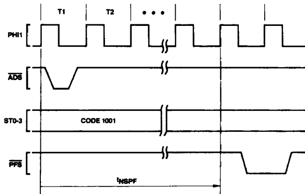
FIGURE 4-19b. Guaranteed Delay, Non-Sequential Fetch to PFS
