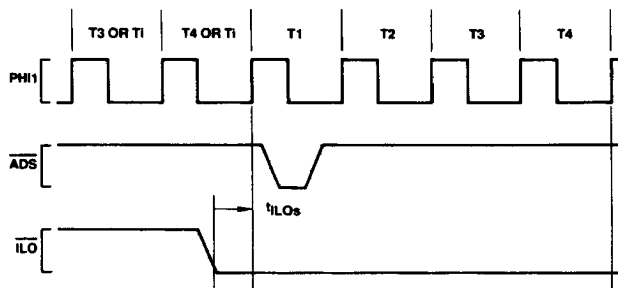
FIGURE 4-20a. Relationship of \overline{\text{ILO}} to First Operand Cycle of an Interlocked Instruction
