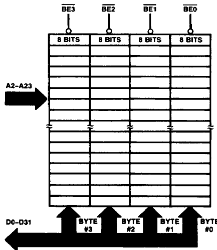
FIGURE 3-11. Memory Interface
