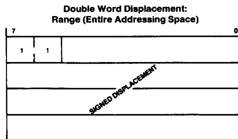
FIGURE 2-8. Displacement Encodings
