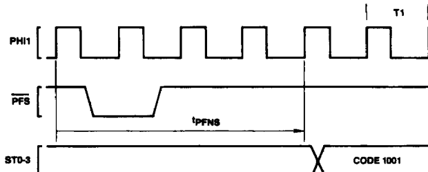
FIGURE 4-19a. Guaranteed Delay, PFS to Non-Sequential Fetch
