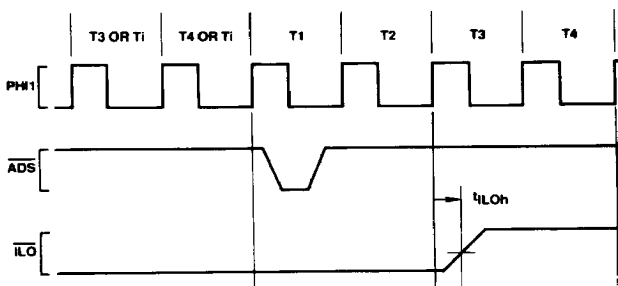
FIGURE 4-20b. Relationship of \overline{\text{ILO}} to Last Operand Cycle of an Interlocked Instruction
