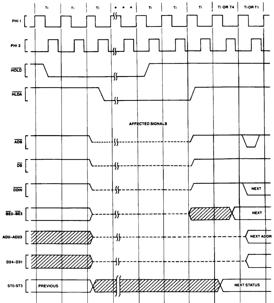
FIGURE 3-20. HOLD Timing, Bus Initially Idle
