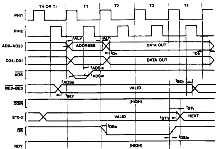
FIGURE 4-4. Write Cycle
