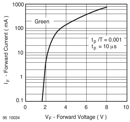
Figure 16. Forward Current vs. Forward Voltage
