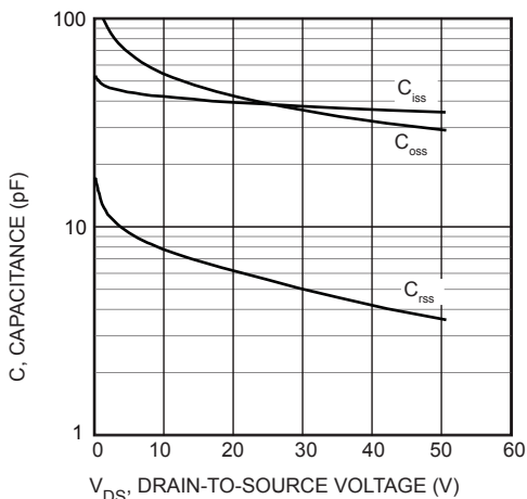
FIGURE 3, Capacitance vs Drain-to-Source Voltage
